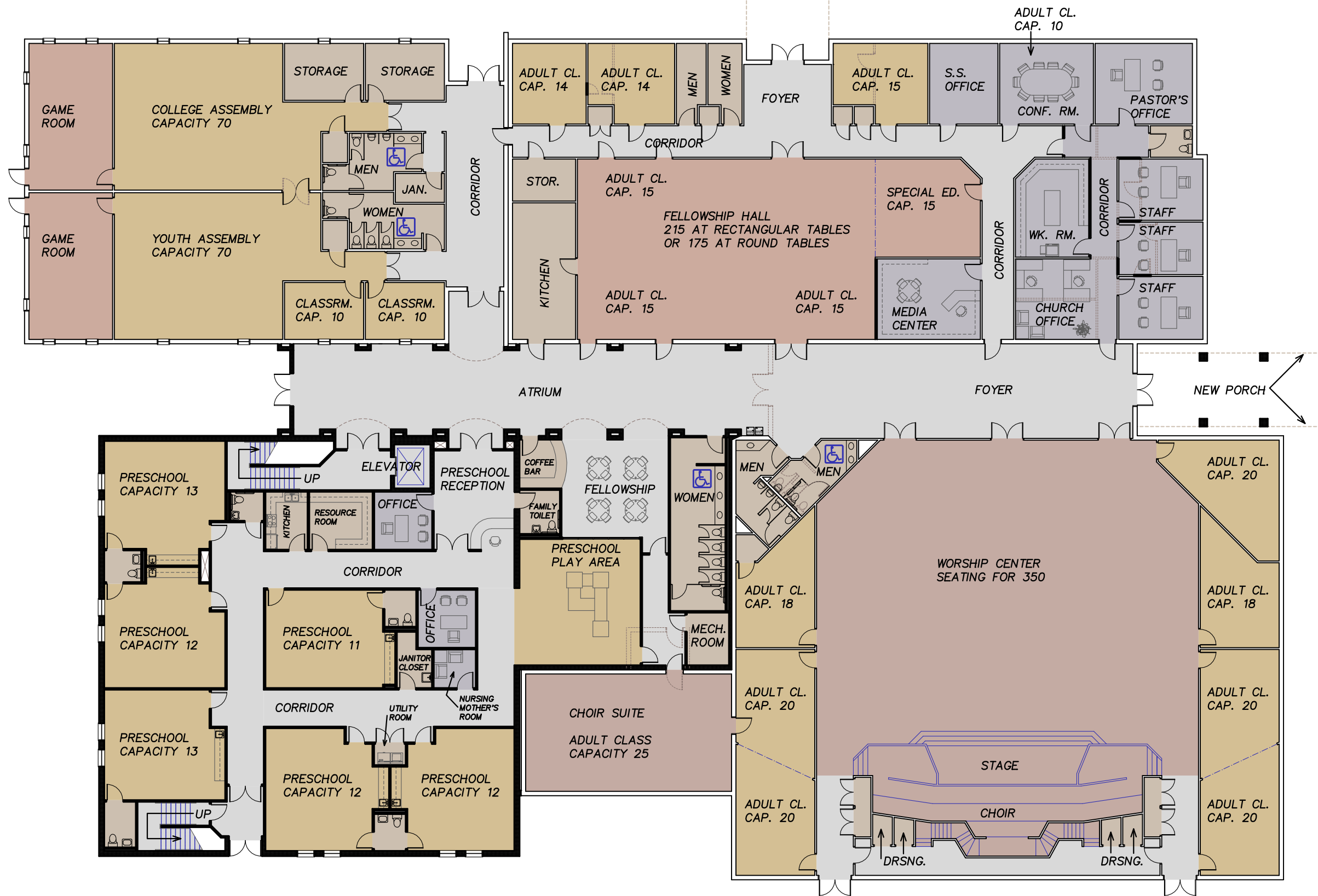
PRELIMINARY FIRST FLOOR PLAN SCALE: 1" = 20'-0"
