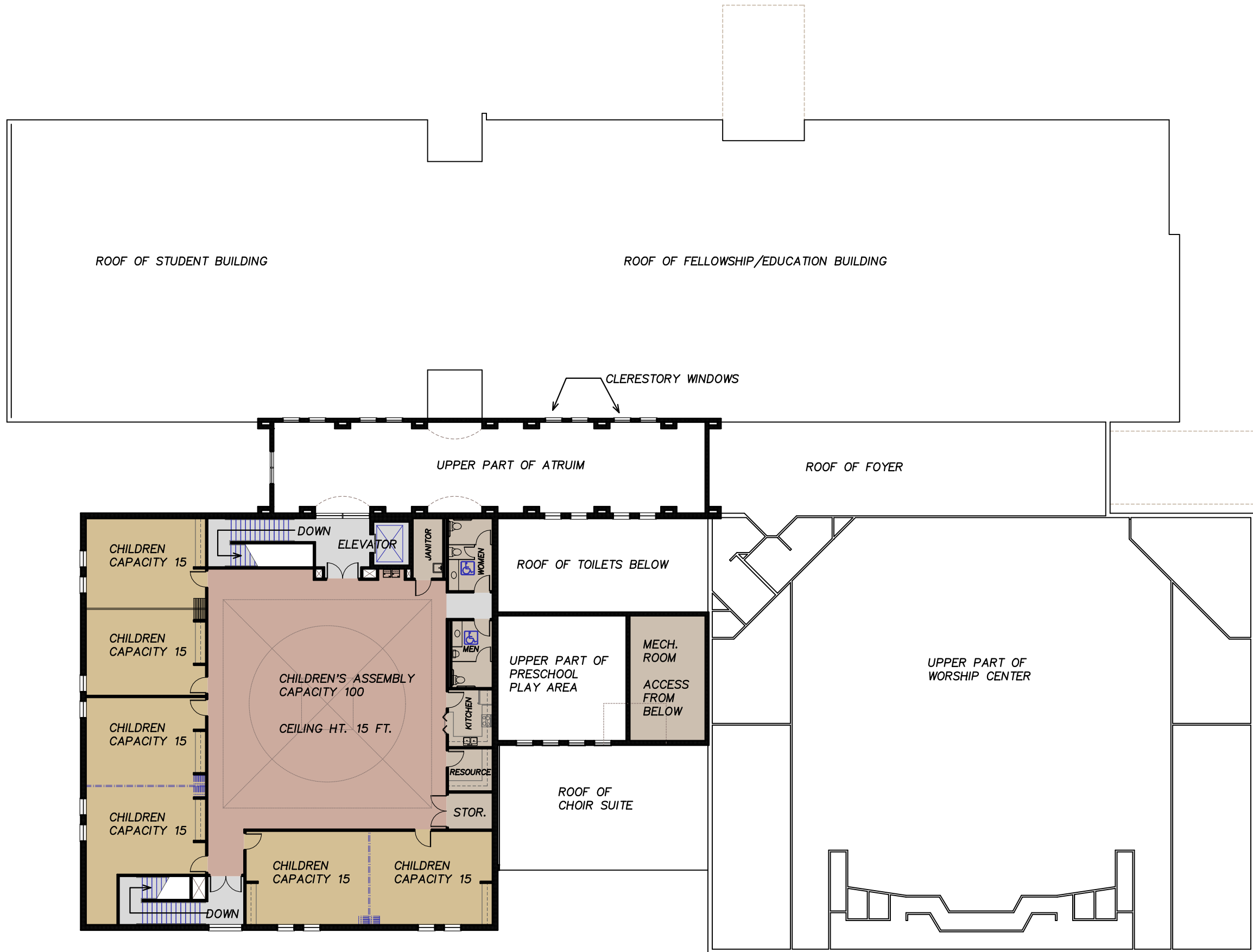
PRELIMINARY SECOND FLOOR PLAN SCALE: 1" = 20'-0"
